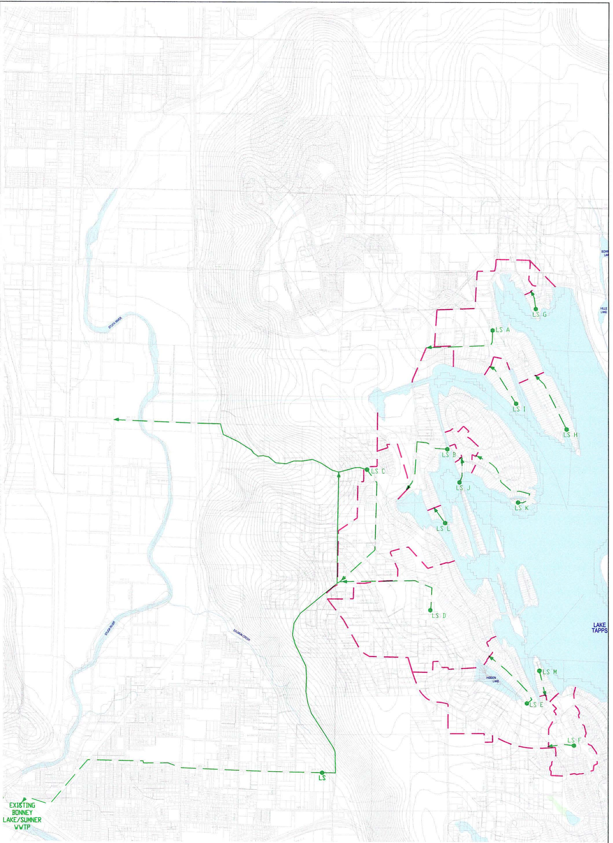
FIGURE 4 CITY OF BONNEY LAKE NORTH SEWER SERVICE AREA SERVICE THROUGH SUMNER
